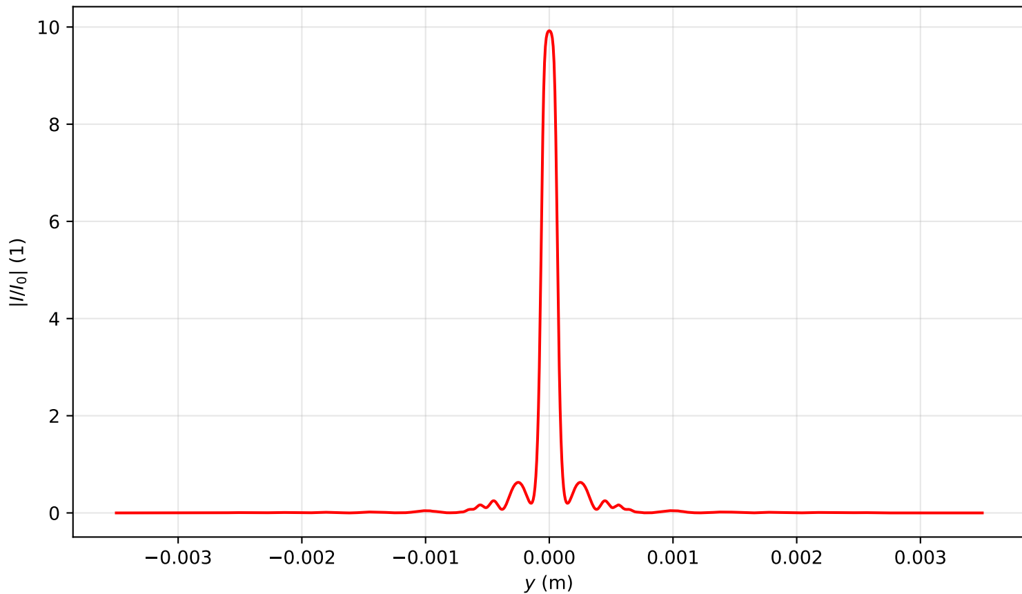
Intensity profile I(x=0, y, z=0.318)/I_0 , \text{Pin}=7.0\text{Pcr} , artificial time
